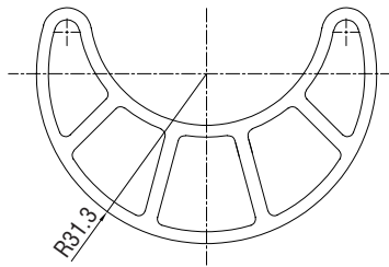
AV-PM-RD-60 Pole Mount Reducer: ø60mm to ø42mm
