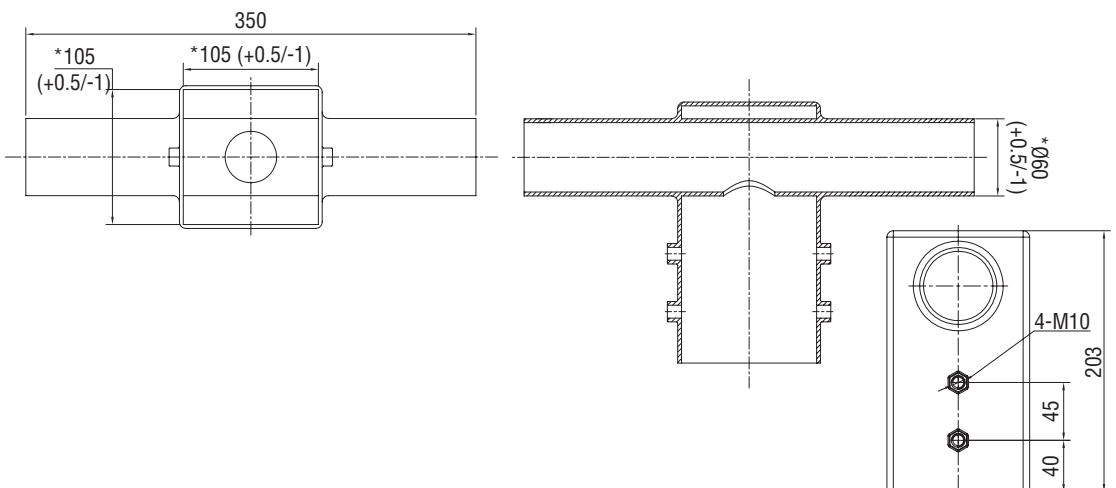
AV-PM-ADT2-SQ Pole Mount 2 Lights Adaptor: 100x100mm
