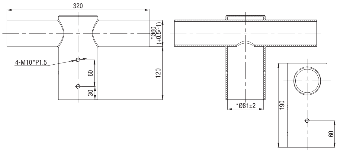
AV-PM-ADT2-76 Pole Mount 2 Lights Adaptor: \varnothing 76\text{mm}
