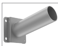
AV-WM-60 Wall Mount Adaptor: ø60mm Spigot
